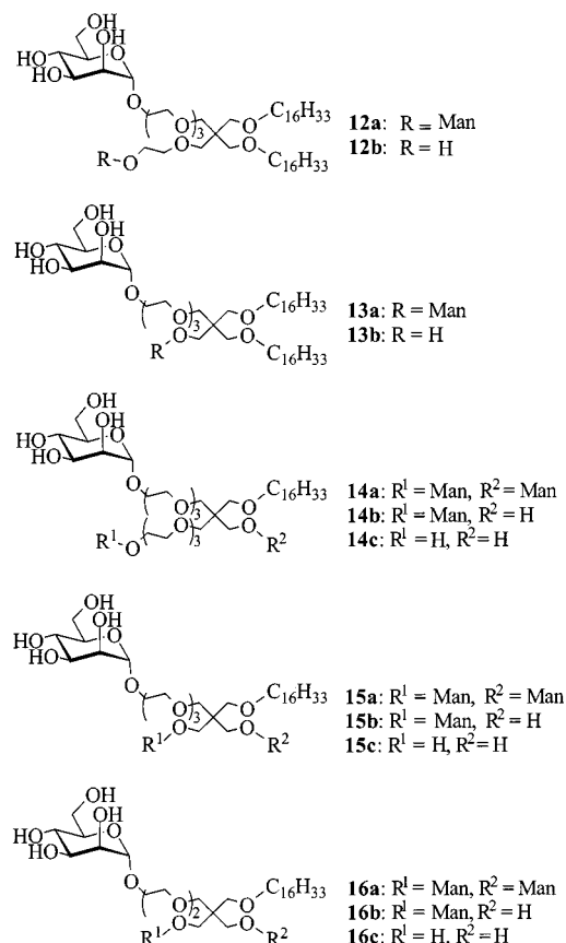
Scheme 4. Different glycosidated mannositides 12 – 16 with variation in the hydrophobic and spacer moieties
