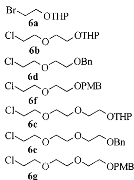
Scheme 2. Halogenated ethyleneoxy derivatives 6a–6g of different lengths with protecting groups as spacer material
