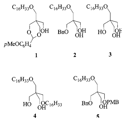
Scheme 1. Different functionalized O -hexadecylpentaerythritol derivatives 1–5
